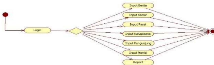
Gambar 4.2.1.2 Activity Diagram Tampilan Administrator
